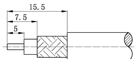
Cable Stripping Dimension
