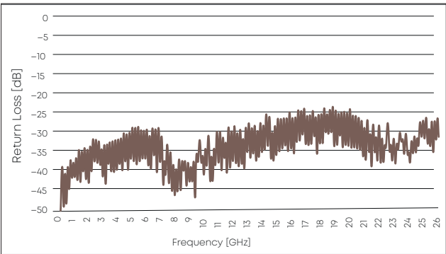
Return loss SUCOFLEX 526V with PC3.5 connectors
