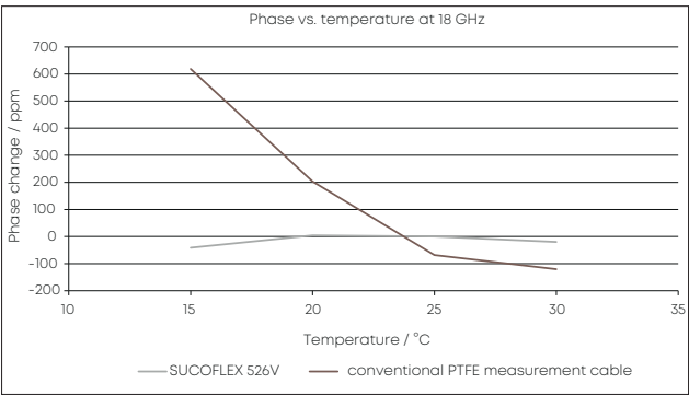
Phase stability vs. temperature performance
