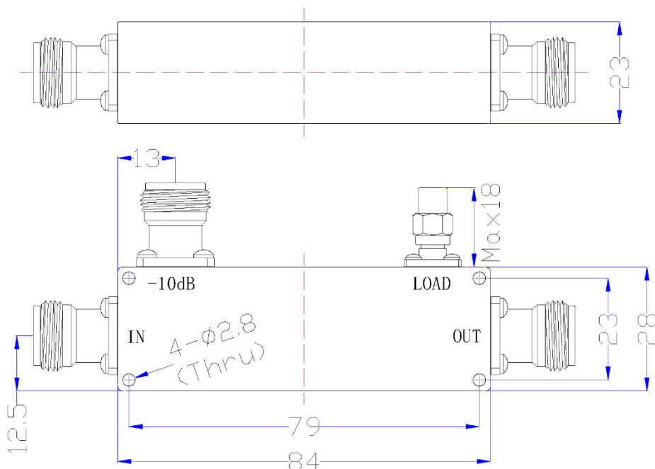
Dimensions (Unit: mm/[inch], Tolerance: ±0.5mm)
