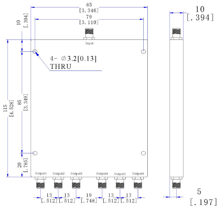
Dimensions (Unit: mm/[inch], Tolerance: ±0.3mm)
