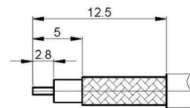
STRIPPING CABLE
