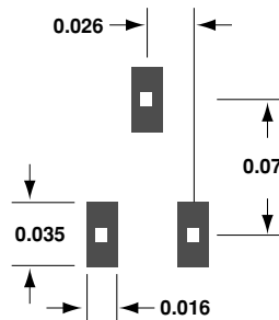
Figure 15. PCB Pad Layout (dimensions in inches).
