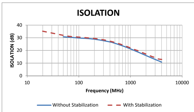
Figure 6 – Isolation
