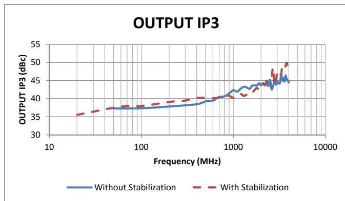
Figure 9 - Output IP3
