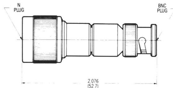
N Plug to BNC Plug
