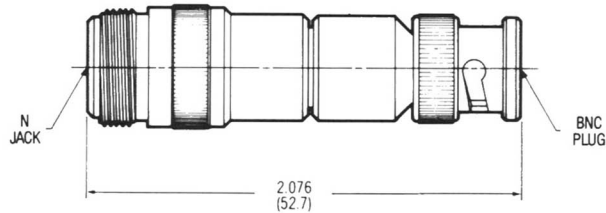
N Jack to BNC Plug
