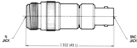
N Jack to BNC Jack
