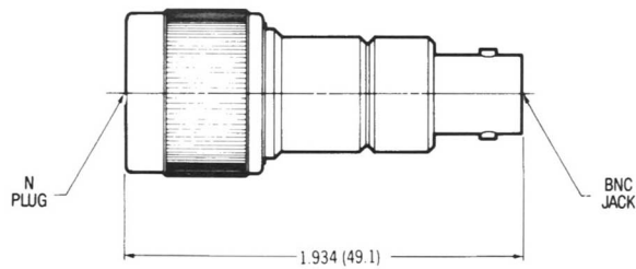
N Plug to BNC Jack
