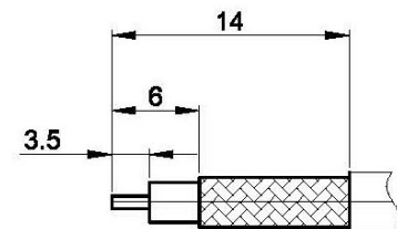
STRIPPING CABLE
