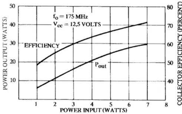
POWER OUT AND EFFICIENCY vs POWER IN
