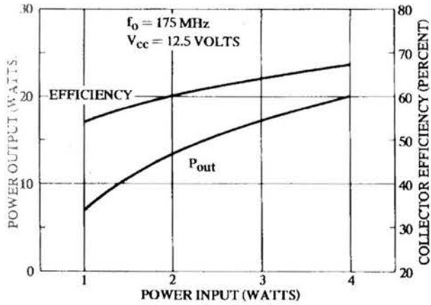
POWER OUT AND EFFICIENCY vs POWER IN
