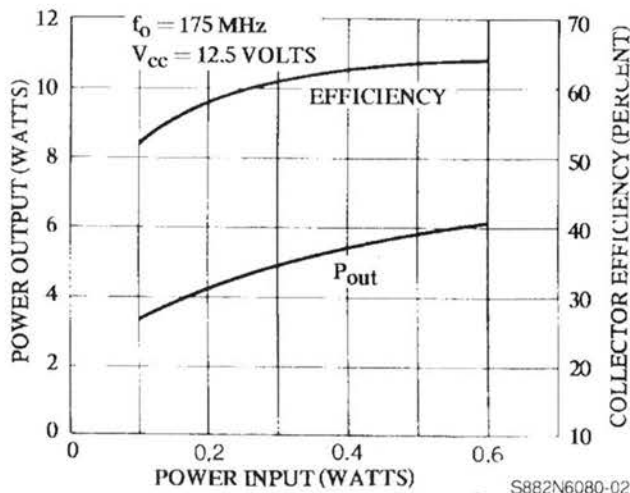
POWER OUT AND EFFICIENCY vs POWER IN
