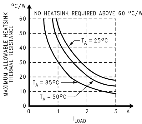
FIGURE 8. Heatsink Thermal Resistance Requirements for Figure 7
