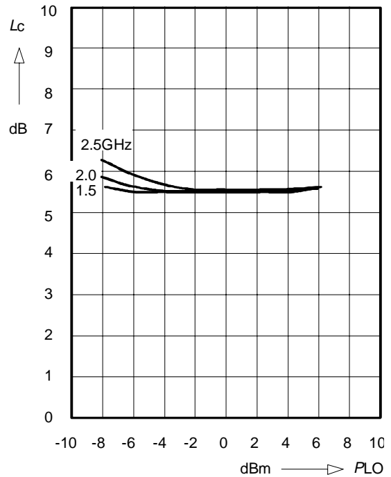
Conversion Loss L_c = f(P_{LO}) V_{DD} = 3V ; f_{IF} = 120\text{MHz} f_{LO} = \text{Parameter}
