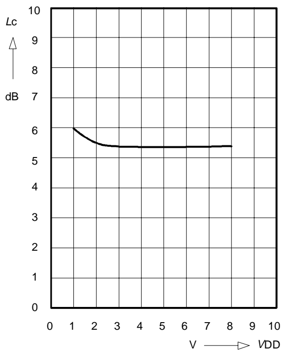
Conversion Loss L_c = f(V_{DD}) P_{LO} = 0\text{dBm} f_{LO} = 1500\text{MHz} ; f_{IF} = 120\text{MHz}
