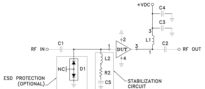
Fig 2b. Evaluation board TB-761-103+ unconditionally stable (see note AN-60-064)
