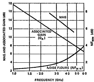
Figure 2. Typical MAG, Noise Figure (NF MIN ) and Associated Gain vs. Frequency (V GR = 10 V, I C = 4 mA), for the HXTR-6101 and HXTR-6102.
