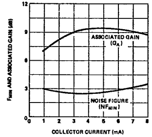
Figure 9. NF_{MIN} and G_A vs. Collector Current at 4 GHz for V_{CE} = 10 V, for the HXTR-6101 and HXTR-6102.
