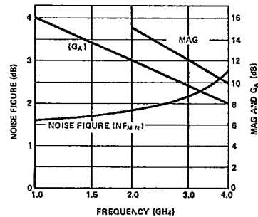
Figure 3. Typical MAG, Noise Figure (NF MIN ) and Associated Gain vs. Frequency (V GR = 10 V, I C = 3 mA), for the HXTR-6103.
