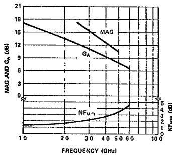
Figure 1. Typical MAG, Noise Figure (NF MIN ), and Associated Gain vs. Frequency (V GR = 10 V, I C = 4 mA), for the HXTR-6001.
