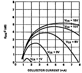
Figure 6. Typical |S_{21}|^2 vs. Bias at 4 GHz, for the HXTR-6101 and HXTR-6102.
