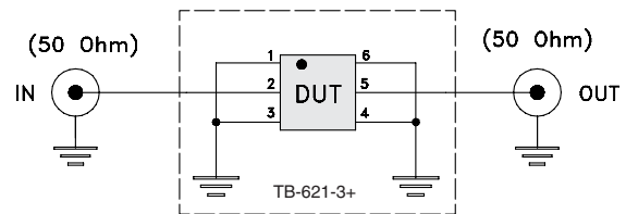
Fig 1. Block diagram of Test Circuit used for characterization, Test board TB-621-3+ Conditions: Attenuation, VSWR: Pin=-10 dBm
