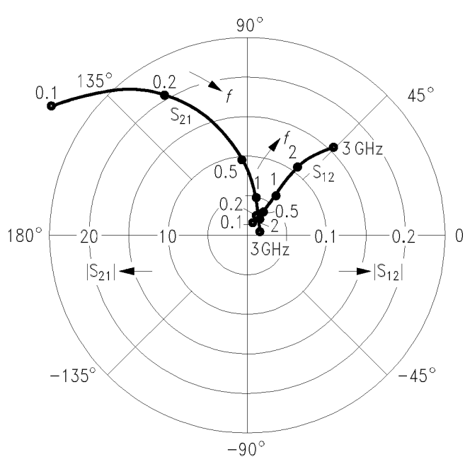
S 12 , S 21 = f ( f )
