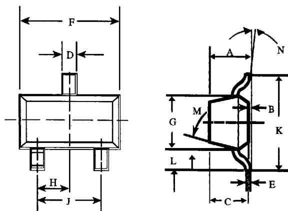
SOT-23 Case Style 287
