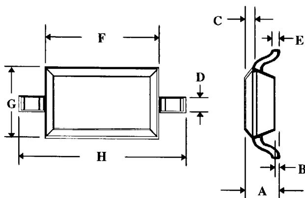
SOD-323 Case Style 1141
