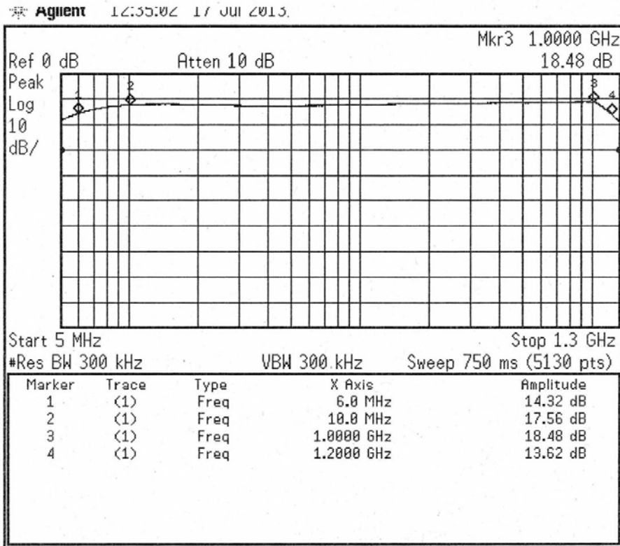
Gain with power supply voltage +13V
