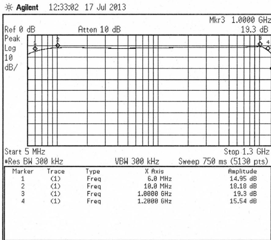
Gain with power supply voltage +24V
