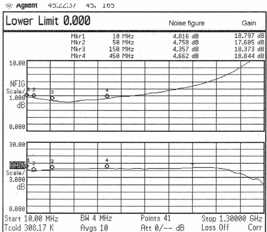
Gain and noise figure with power supply voltage +24V
