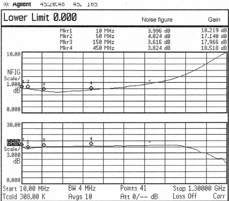
Gain and noise figure with power supply voltage +13V
