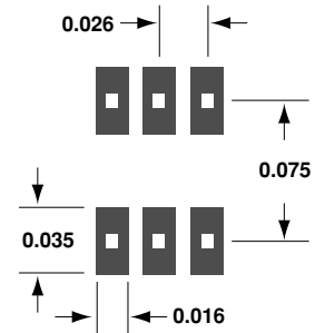
Figure 21. PCB Pad Layout (dimensions in inches).
