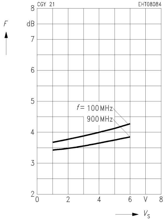
Noise figure F = f(V_s) R_s = R_L = 50 \Omega
