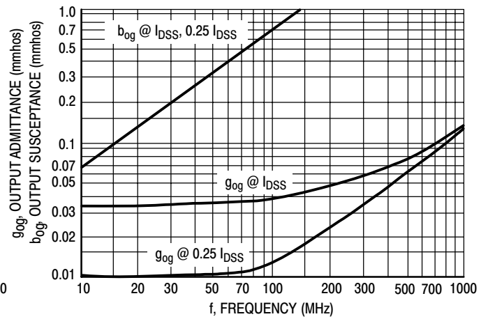
Figure 12. Output Admittance ( y_{og} )
