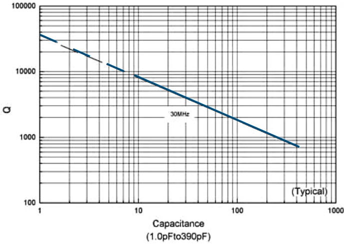
Q vs.Capacitance
