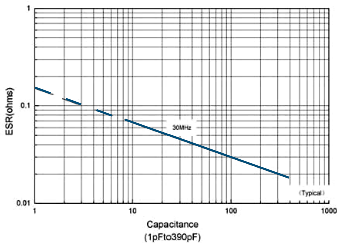
ESR vs.Capacitance
