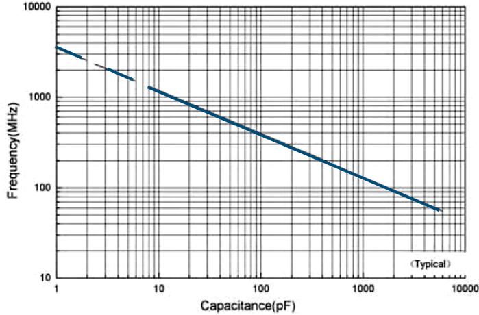
Resonance vs.Capacitance
