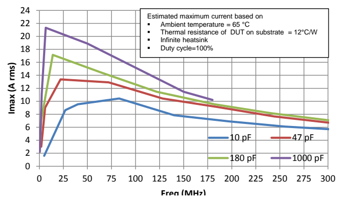
Maximum Current vs Frequency: 3838/S58E
