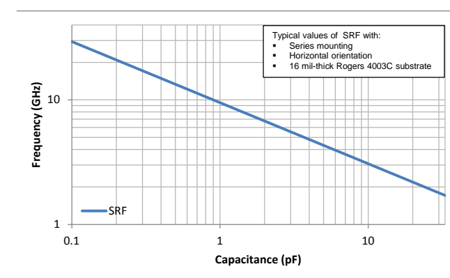
Resonant Frequency : 0402/R07S
