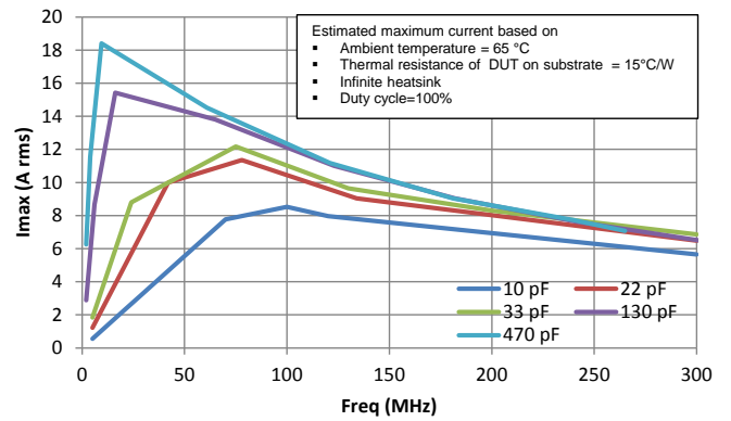
Maximum Current vs Frequency: 2525/S48E
