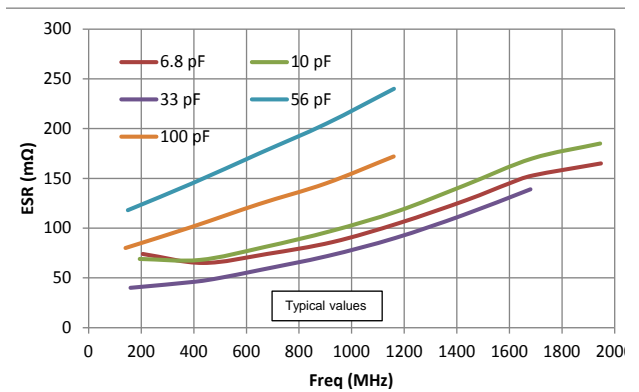
Equivalent Series Resistance: 0201/R05L
