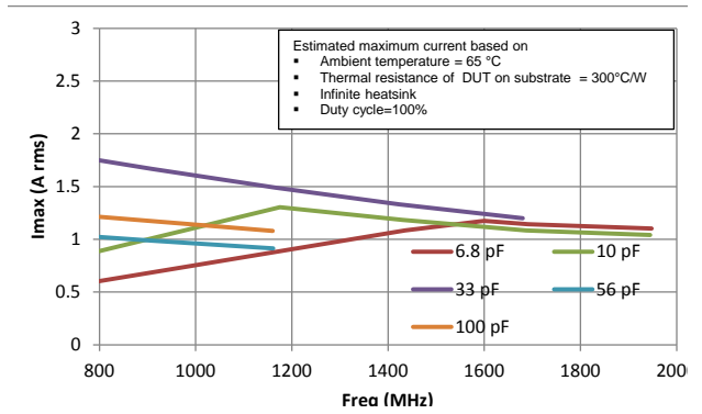
Maximum Current vs Frequency: 0201/R05L
