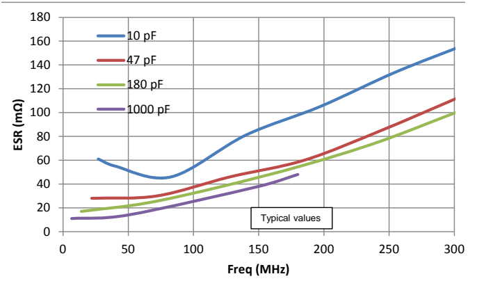
Equivalent Series Resistance: 3838/S58E
