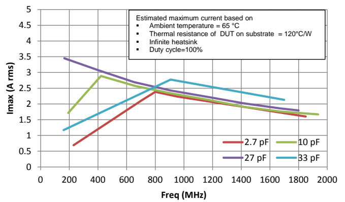
Maximum Current vs Frequency: 0402/R07S
