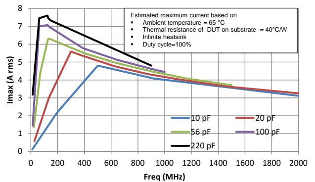
Maximum Current vs Frequency: 0805/R15S
