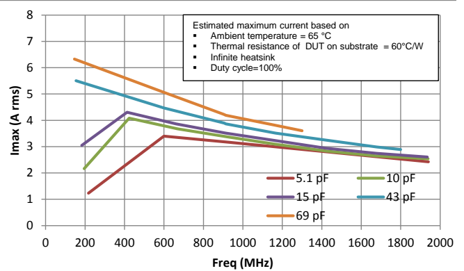
Maximum Current vs Frequency: 0603/R14S
