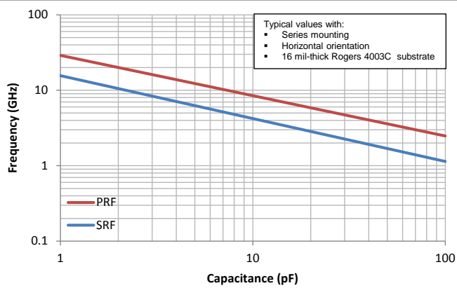
Resonant Frequency : 0603/R14S
