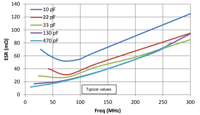
Equivalent Series Resistance: 2525/S48E
