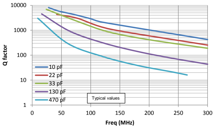
Q factor: 2525/S48E
