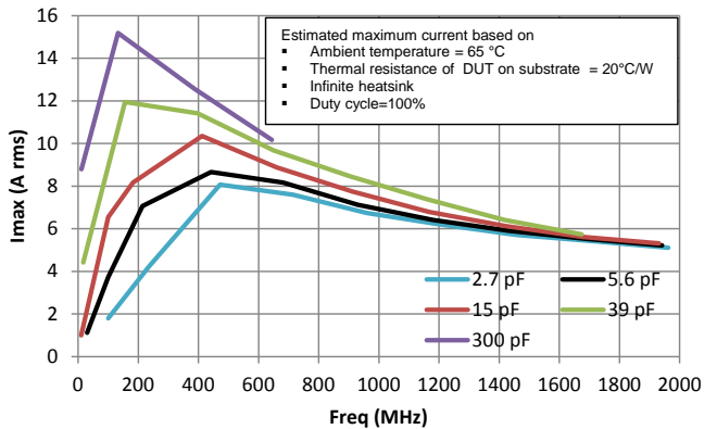
Maximum Current vs Frequency: 1111/S42E
